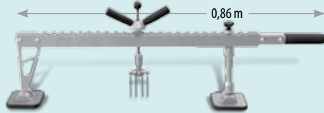
Levelling bar double action 053564 (p.10)
